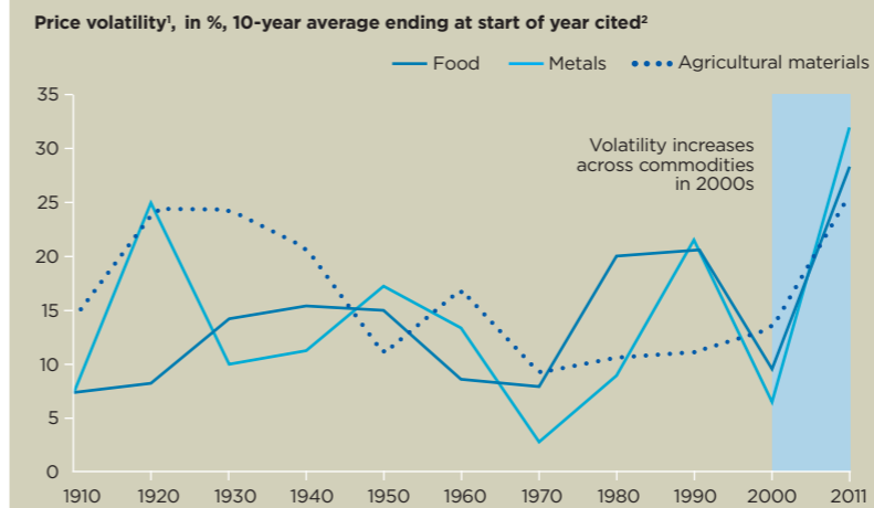
FIGURE 5 Price volatility has risen above long-term trends in recent decades Price volatility 1 , in %, 10-year average ending at start of year cited 2
